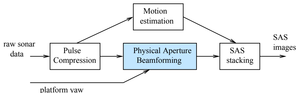
Figure 6 : Processing stages for a Synthetic Aperture Sonar
