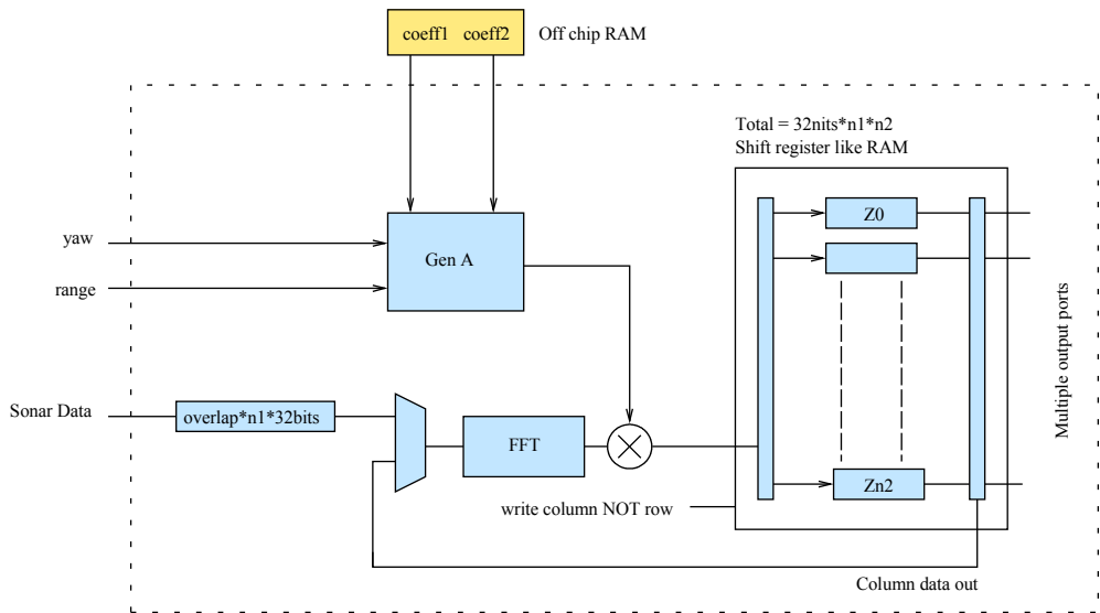
Figure 4 FPGA architecture of Yaw stabilised physical aperture beamformer
