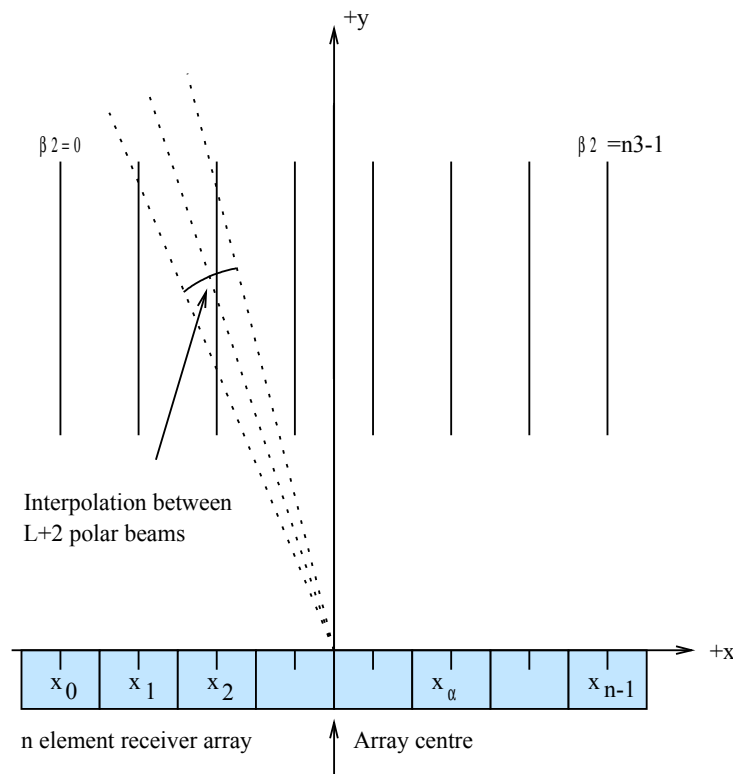
Figure 3 : beams output from polar interpolator – example shows parallel beams
