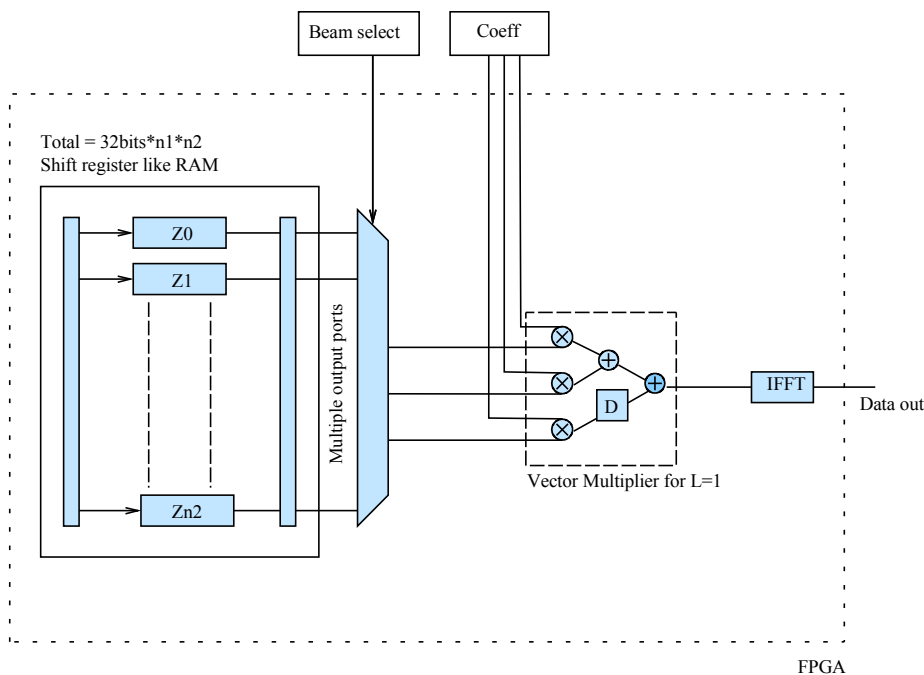
Figure 5 : FPGA Architecture for polar interpolation.
