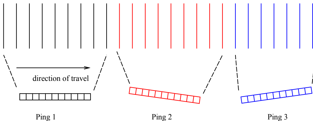
Figure 8 Sonar image formed from multi beam sonar
