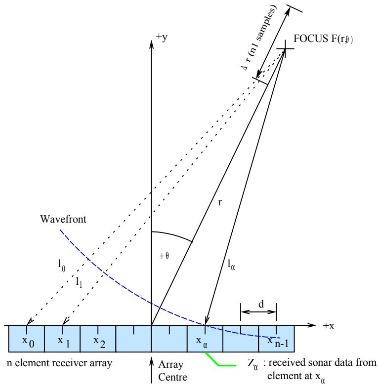
Figure 1 : Near field arrival at receiver array from a sector about broadside
