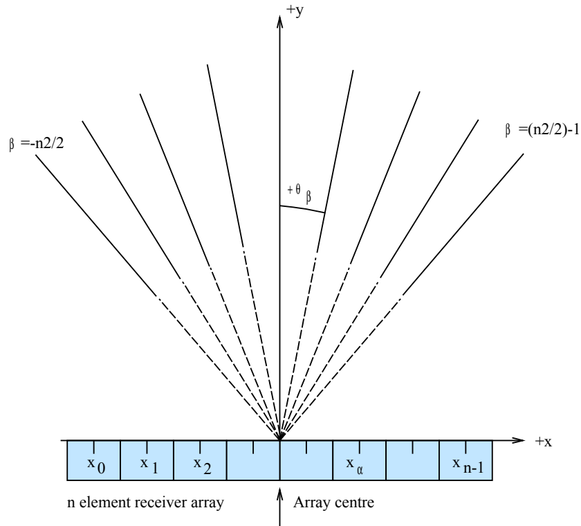
Figure 2 : Polar beams formed by polar beamformer
